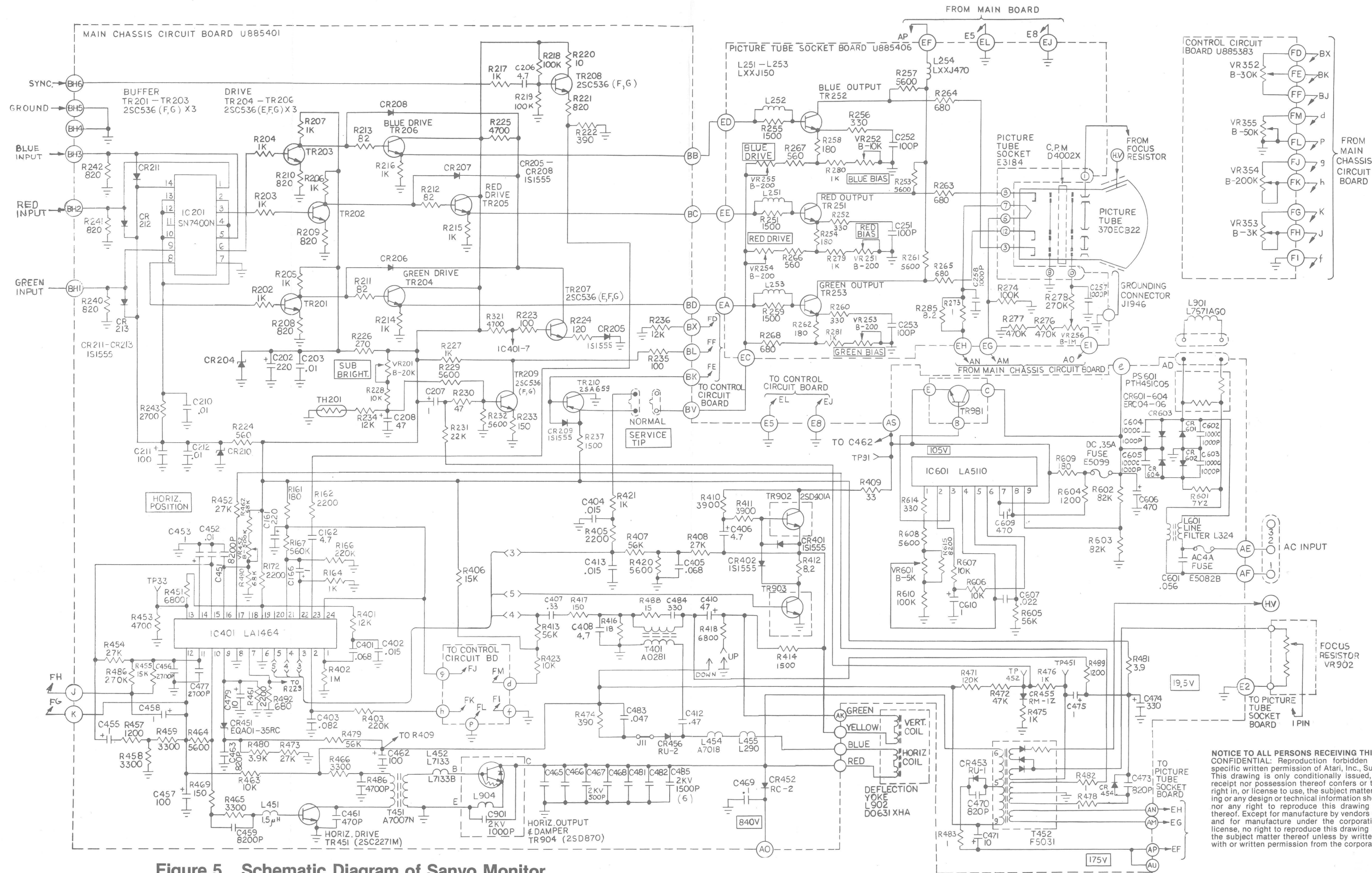
Figure 5 Schematic Diagram of Sanyo Monitor
