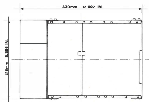
CHASSIS WITH SWITCH MODEL POWER SUPPLY INCORPORATED
