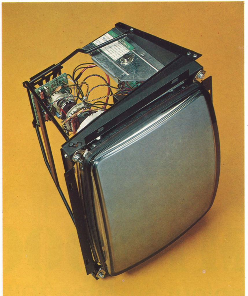
MTC 900.E colour monitor 20'' vertical position
