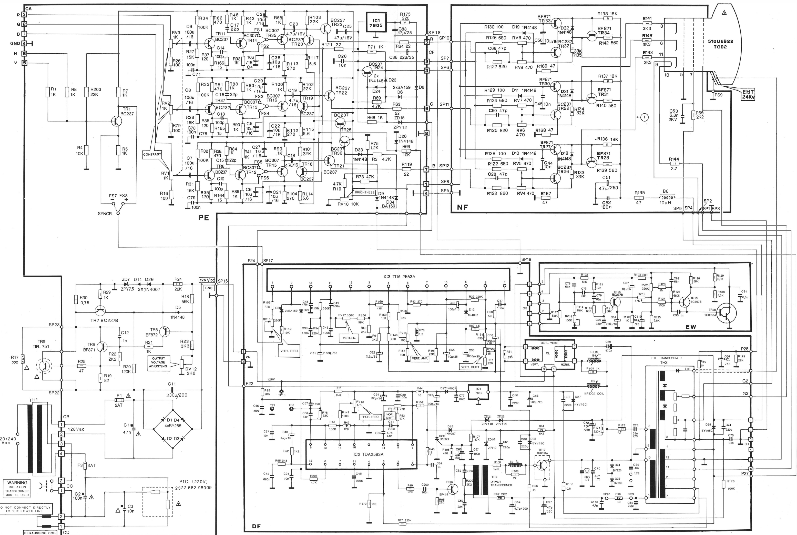
MTC900/E SCHEMATIC DIAGRAM
