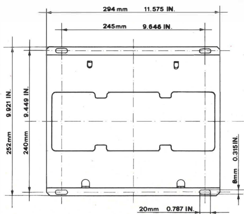
SUPPORT FOR CHASSIS ASSEMBLY
