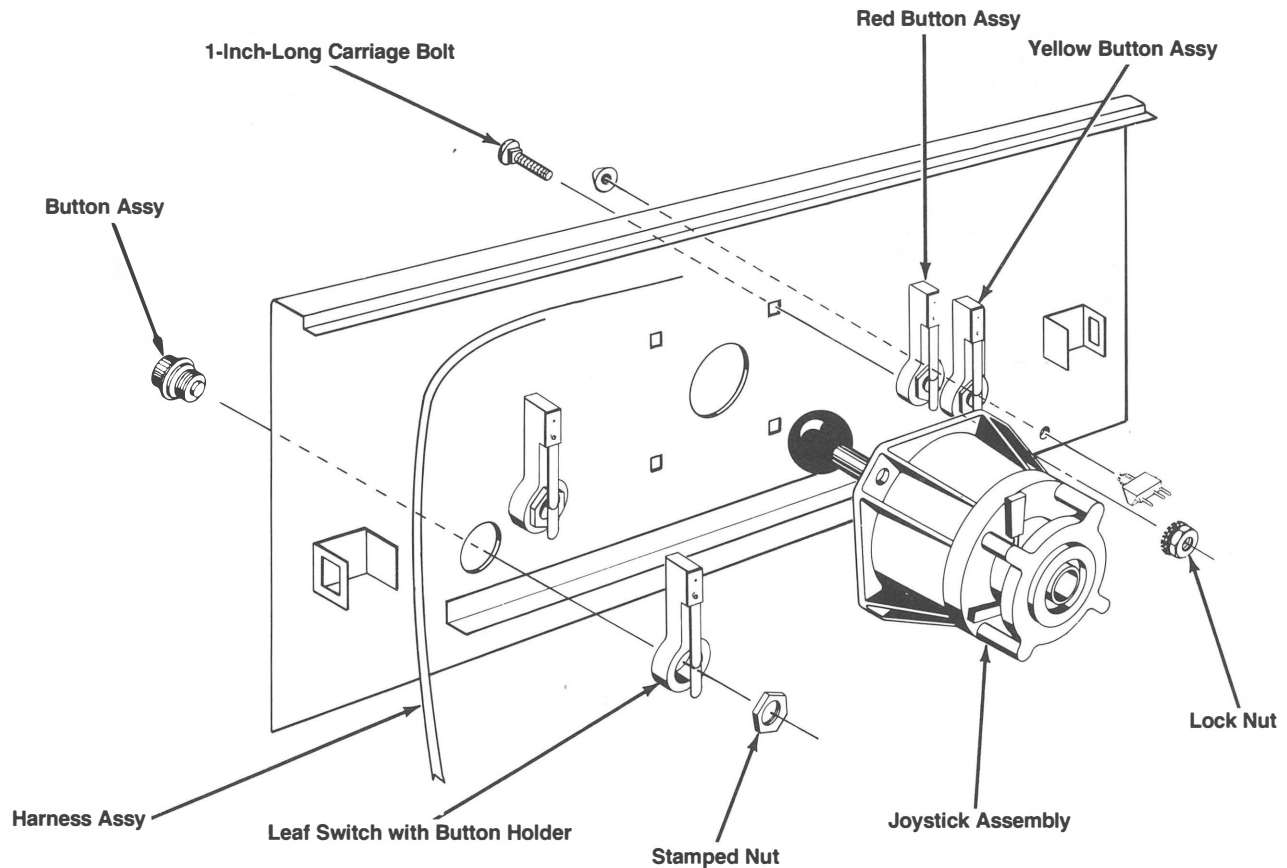
Figure 3-1 Leaf Switch and Joystick Removal
