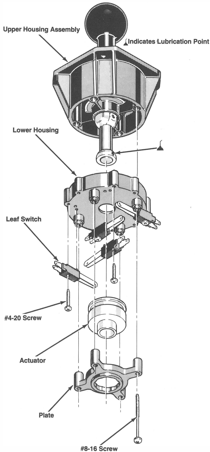
Figure 3-2 Joystick Lubrication
