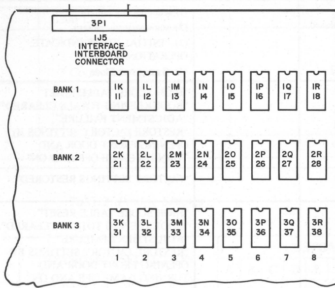
Figure 3. RAM Location and Numbering on CPU Board (see above)
