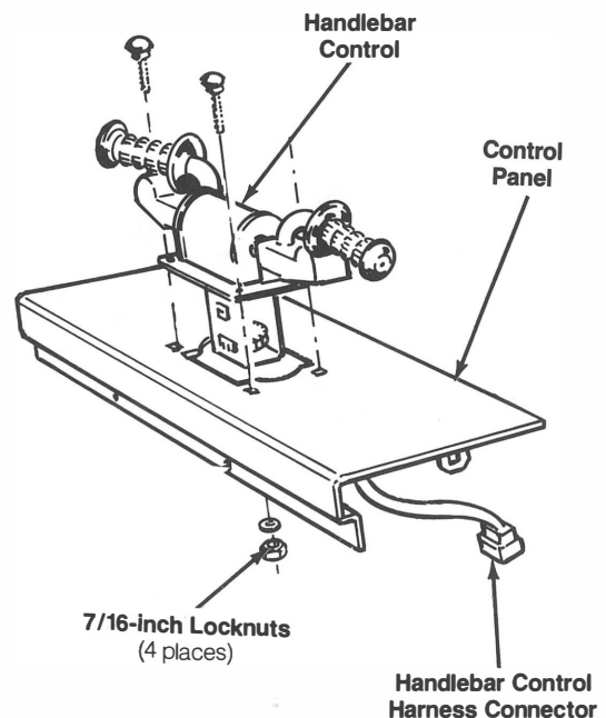
Figure 3-6 Handlebar Control Removal
