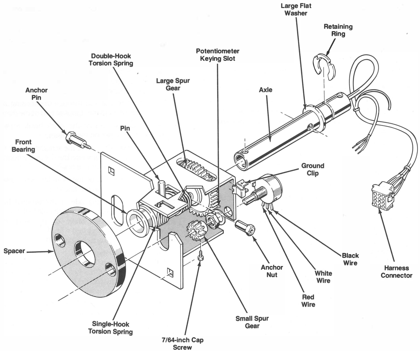
Figure 3-9 Steering Unit Disassembly/Reassembly
